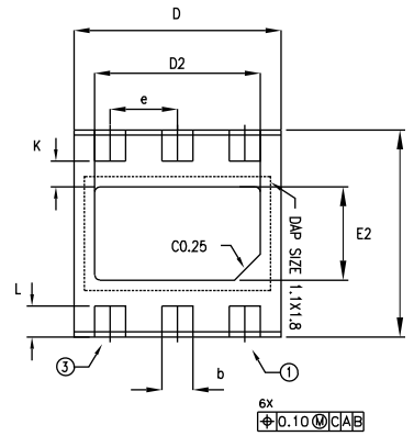
Figure 28. DFN6 (2 x 2) wettable flanks package outline
