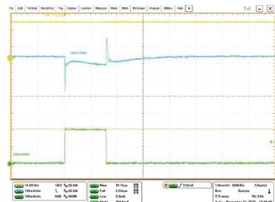
Figure 16. Load transient V_{EN}=1V
