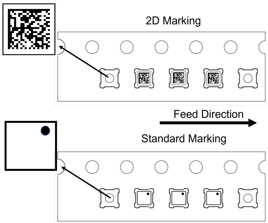
Figure 35. Pin 1 orientation
