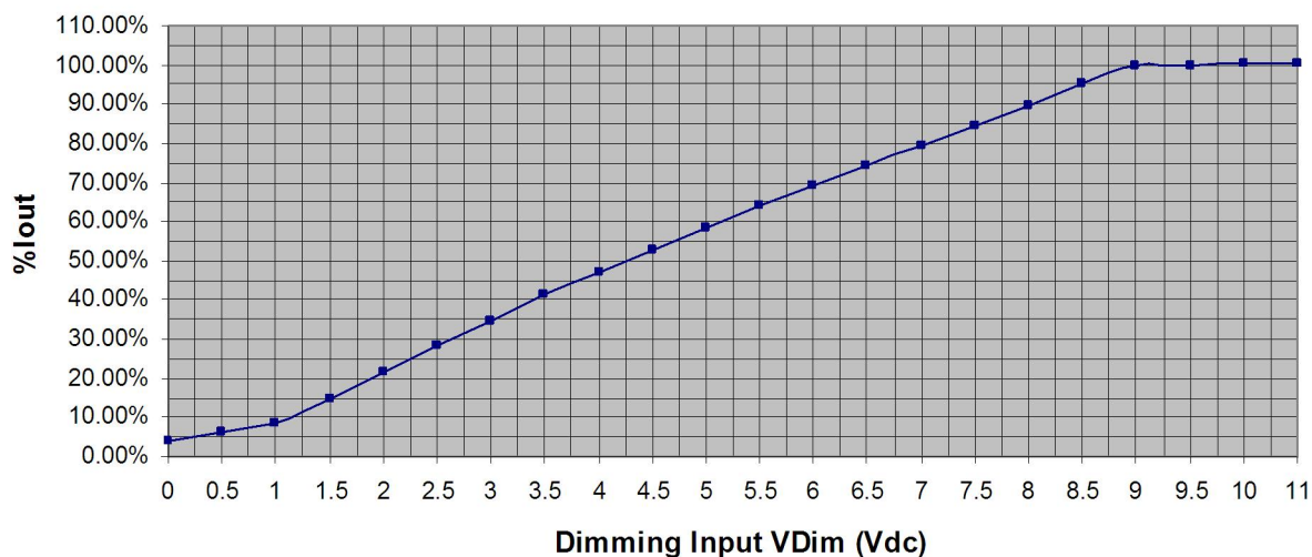
% Output Current vs. 0-10VDC Dimming Input
