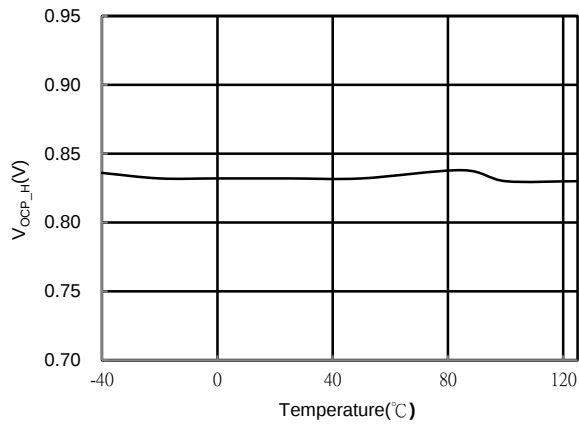
Fig. 7 V_{OCP\_H} vs. Temperature
