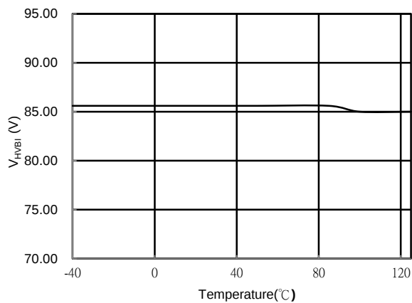
Fig. 11 V_{HVBI} vs. Temperature
