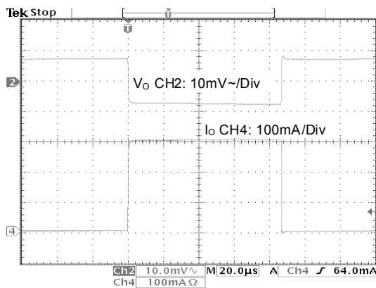
Fig.12 Load Transient Response( C_O=4.7\mu F )
