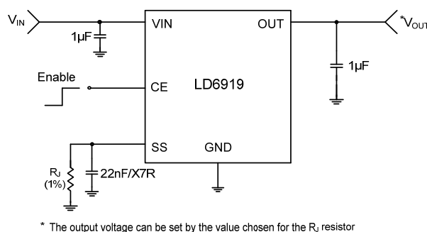
Fig. 1 Typical Application Circuit for General Purpose
