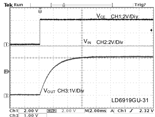
Fig.4 Start Up Waveform Ccss=22nF
