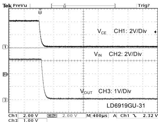
Fig.5 EN Pin Shutdown Response
