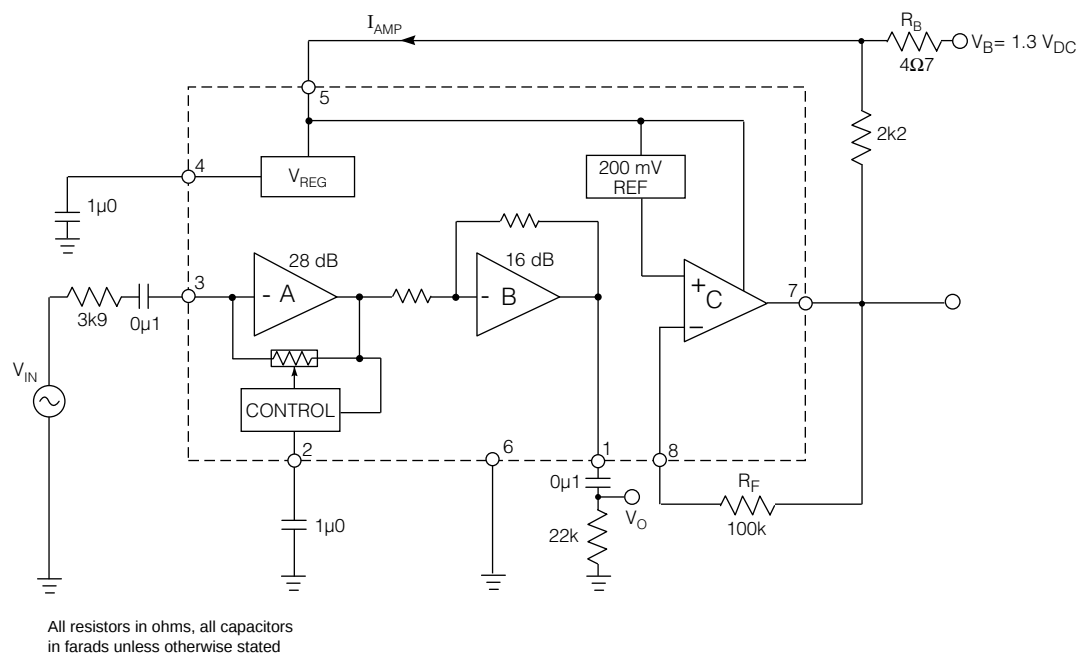
Fig. 1 Test Circuit
