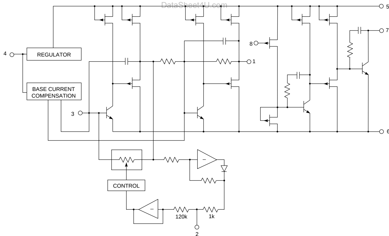
Fig. 2 Functional Schematic
