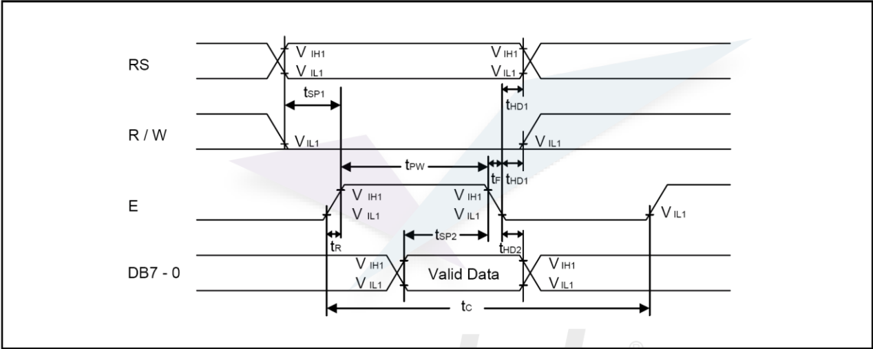
Timing Diagram Writing mode
