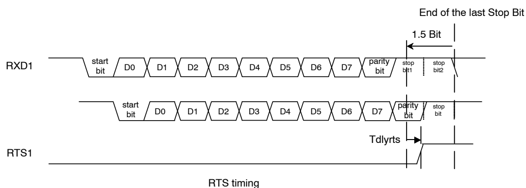
Figure 36. RTS Timing
