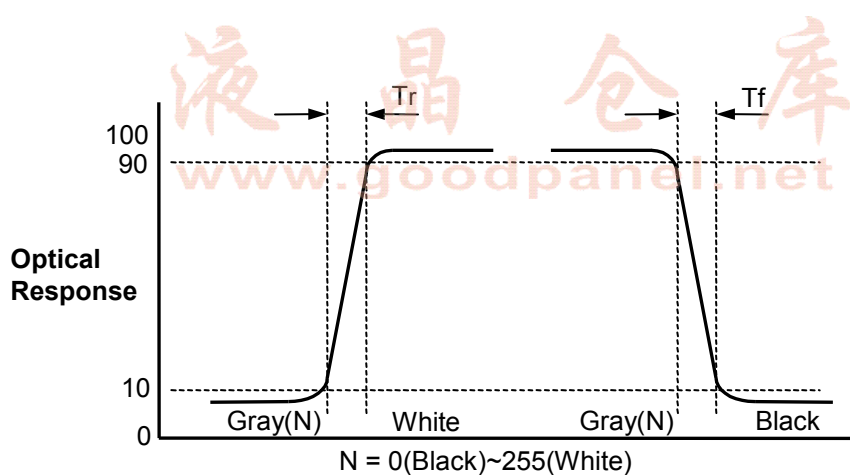
FIG. 3 Response Time
