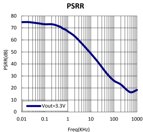
4) Ripple rejection vs. Frequency
