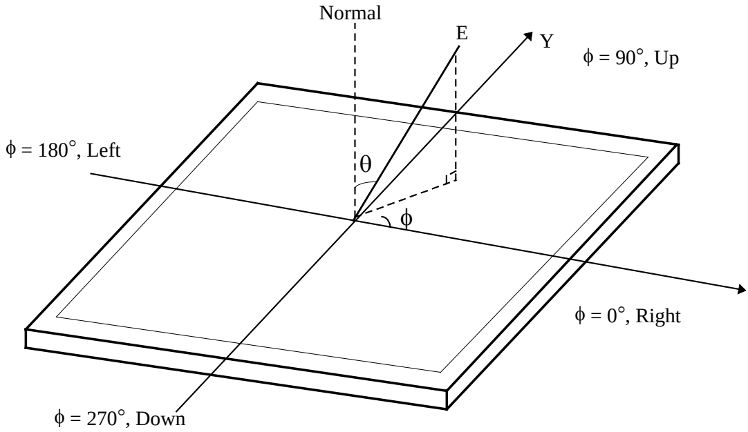
FIG. 4 Viewing Angle
