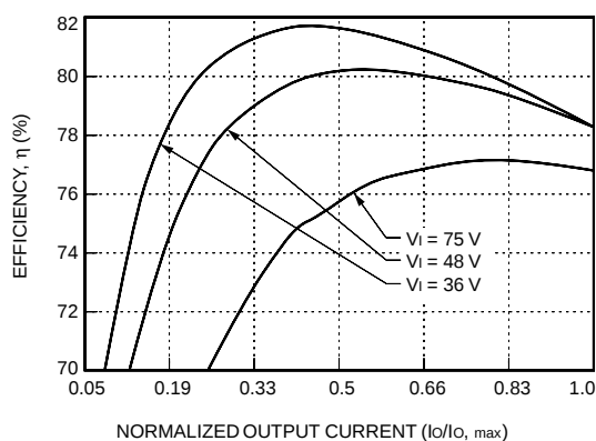
Figure 23. LW015B, C Typical Efficiency vs. Normalized Output Current at T_c = 25^\circ\text{C}
