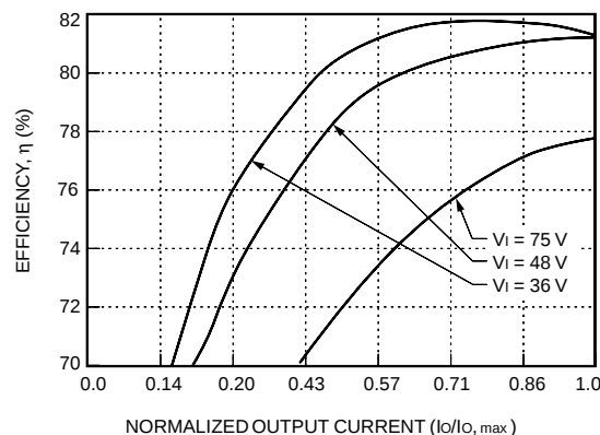
Figure 26. LW010A, B, C Typical Efficiency vs. Normalized Output Current at T_c = 25^\circ\text{C}
