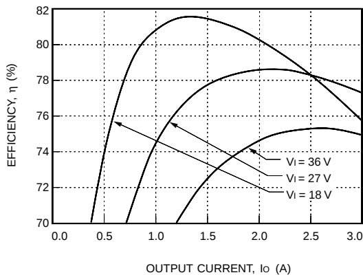
Figure 18. LC015F Typical Efficiency vs. Output Current at T_c = 25^\circ\text{C}
