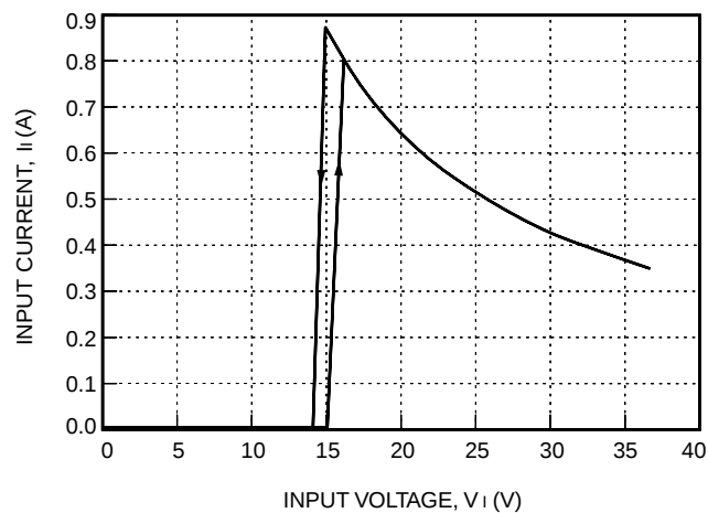
Figure 1. LC010 Input Current vs. Input Voltage at I o = I o, max and T c = 25 °C
