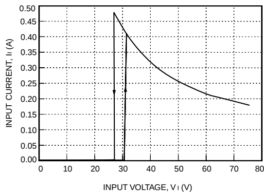
Figure 3. LW010 Input Current vs. Input Voltage at I_o = I_{o, \max} and T_c = 25^\circ\text{C}
