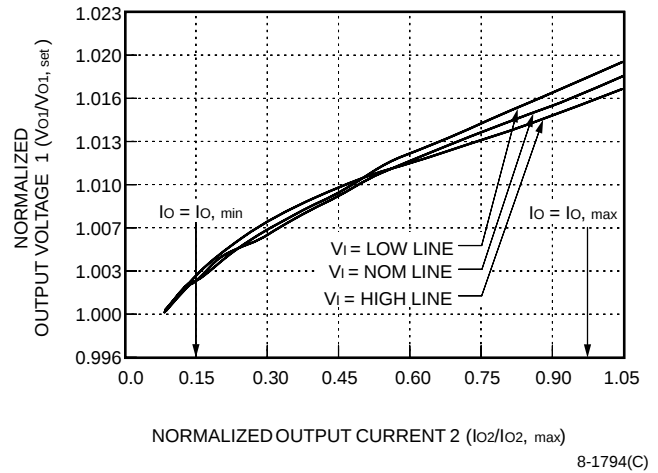
Figure 10. Lx010BK, CL Typical Cross Regulation, Normalized Vo_1 vs. Normalized Io_2 with Fixed Io_1 = Io, \min at T_c = 25^\circ\text{C}
