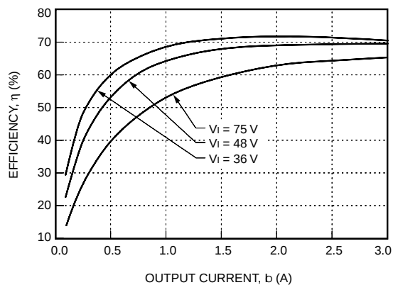
Figure 24. LW010D, 015D Typical Efficiency vs. Output Current at T_c = 25^\circ\text{C}
