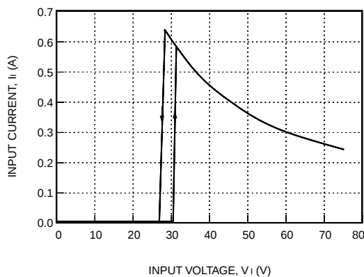
Figure 4. LW015 Input Current vs. Input Voltage at I_o = I_{o, \max} and T_c = 25^\circ\text{C}
