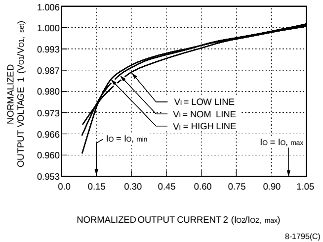
Figure 11. Lx010BK, CL Typical Cross Regulation, Normalized Vo_1 vs. Normalized Io_2 with Fixed Io_1 = Io, \max at T_c = 25^\circ\text{C}
