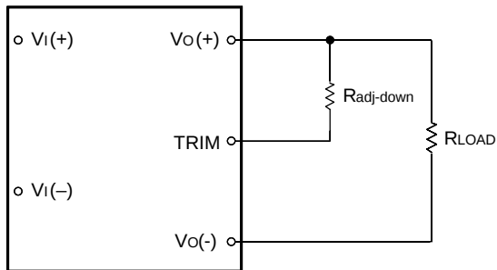
Figure 39. Circuit Configuration to Decrease Output Voltage
