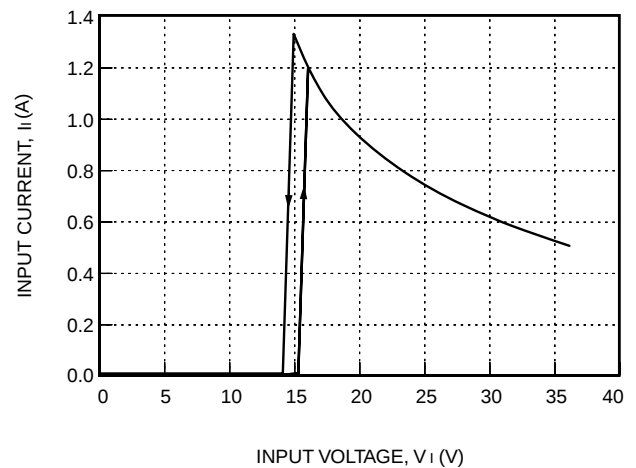
Figure 2. LC015 Input Current vs. Input Voltage at I o = I o, max and T c = 25 °C
