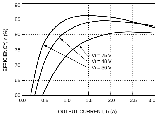
Figure 22. LW015A Typical Efficiency vs. Output Current at T_c = 25^\circ\text{C}
