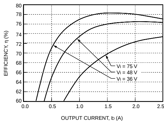
Figure 27. LW010F Typical Efficiency vs. Output Current at T_c = 25^\circ\text{C}
