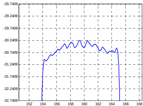
Passband Response
