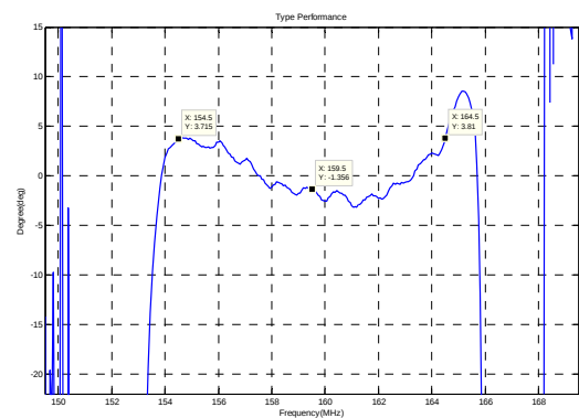
Phase Linearity(f0±5MHz)
