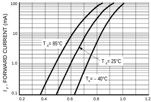
Figure 1. Forward Voltage
