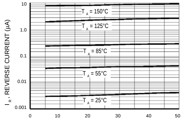
Figure 2. Leakage Current
