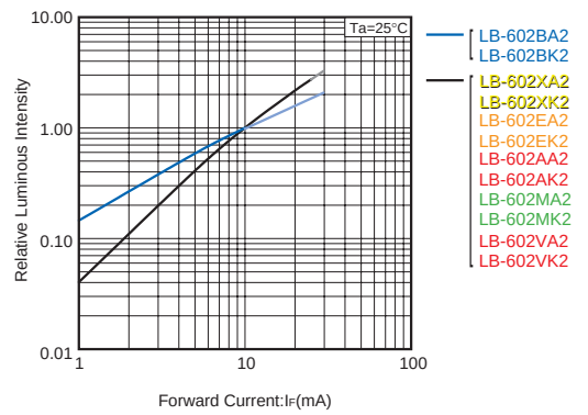
Fig.2 Relative Luminous Intensity - Forward Current
