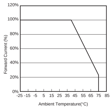
Fig.7 Derating
