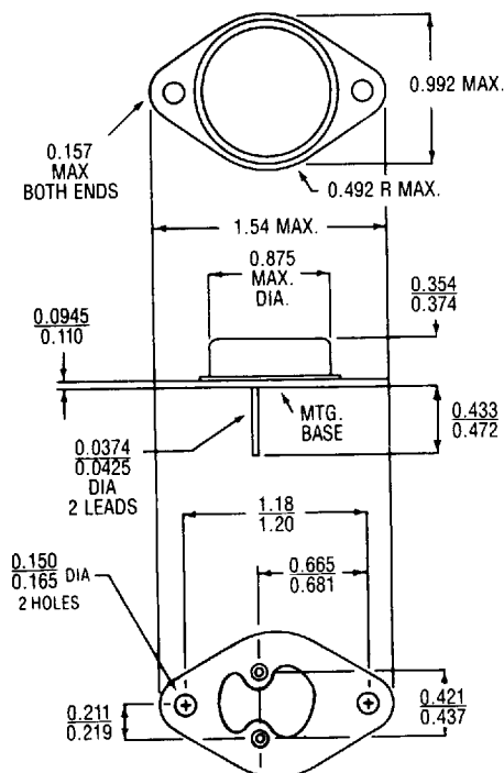
TO-3 (COPPER/STEEL)
