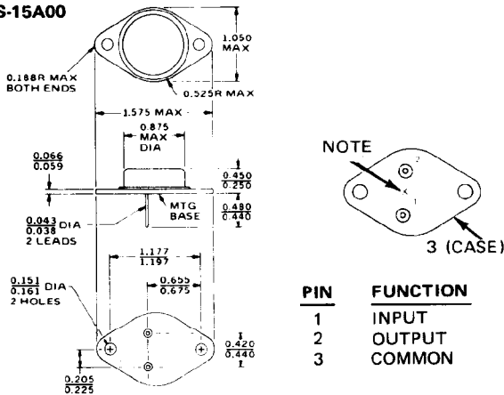
LAS-1500 LAS-15A00 TO-3 3-TERMINAL (STEEL)
