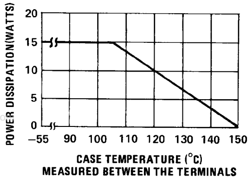
POWER DERATING
