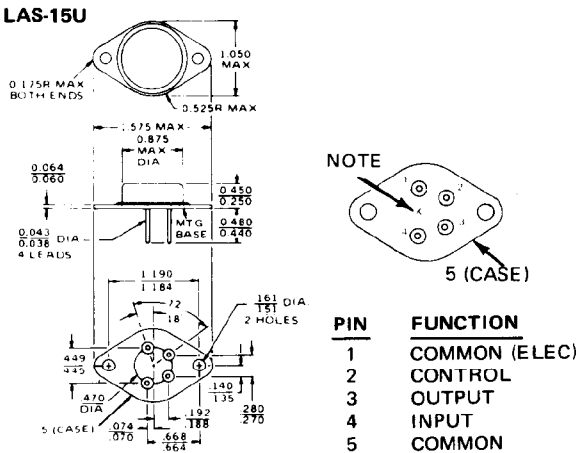
TO-3 4-TERMINAL (STEEL)
