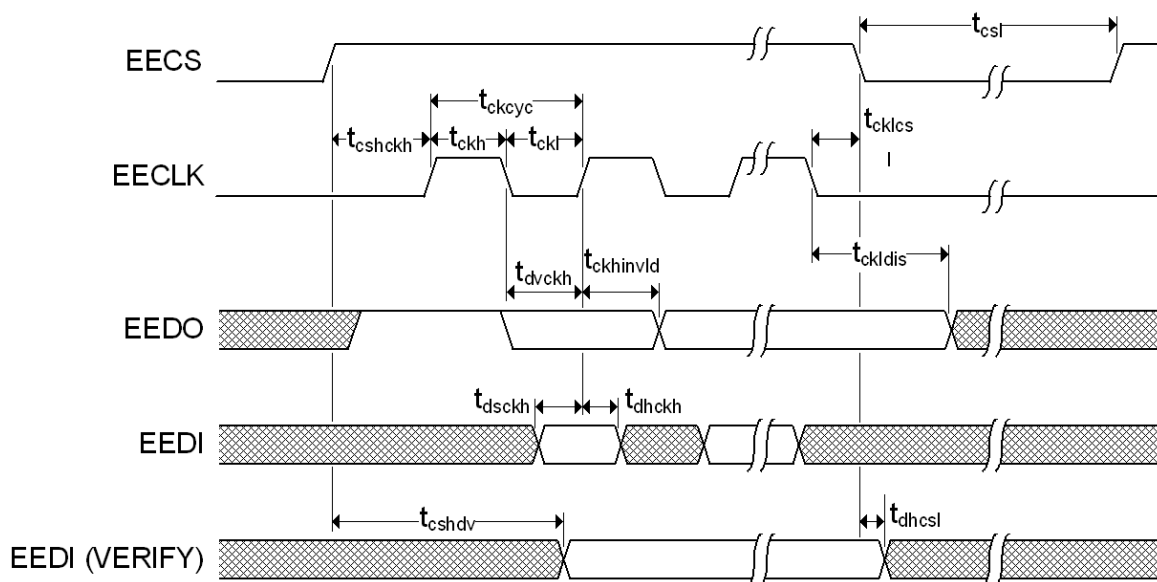
Figure 7.5 EEPROM Timing
