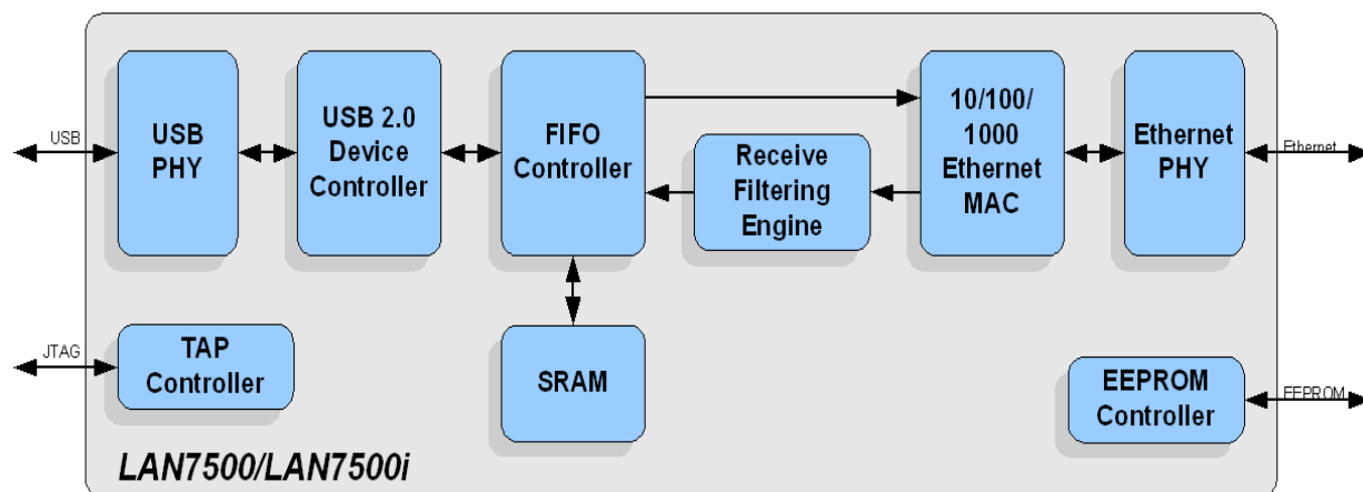
Figure 1.1 LAN7500/LAN7500i System Diagram
