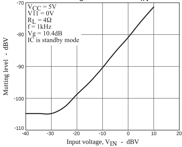
Mutting attenuation - V_{IN}
