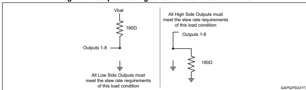
Figure 4. Output loading for slew rate measurements
