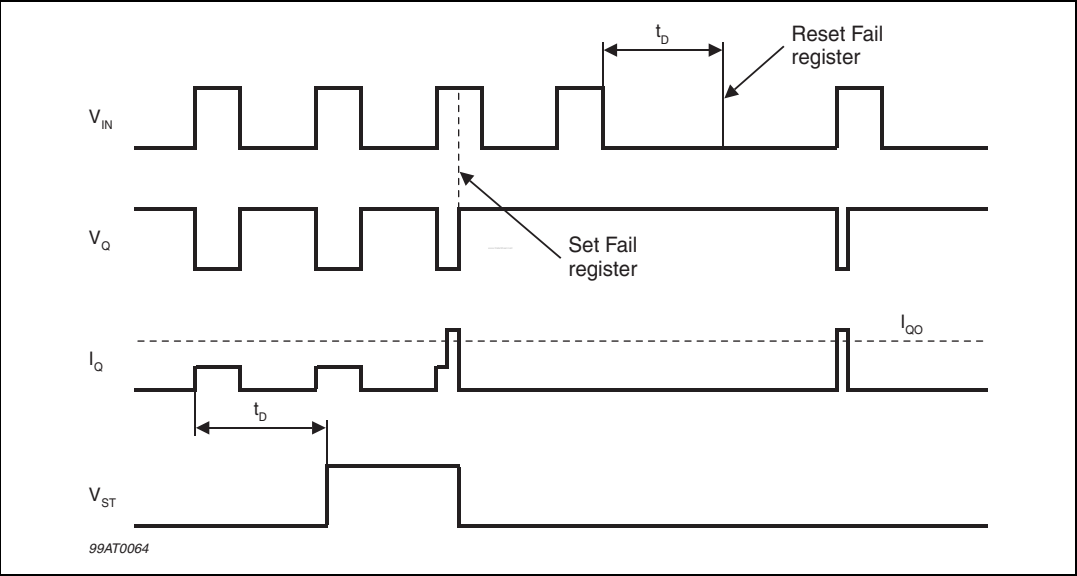
Figure 8. Current overload
