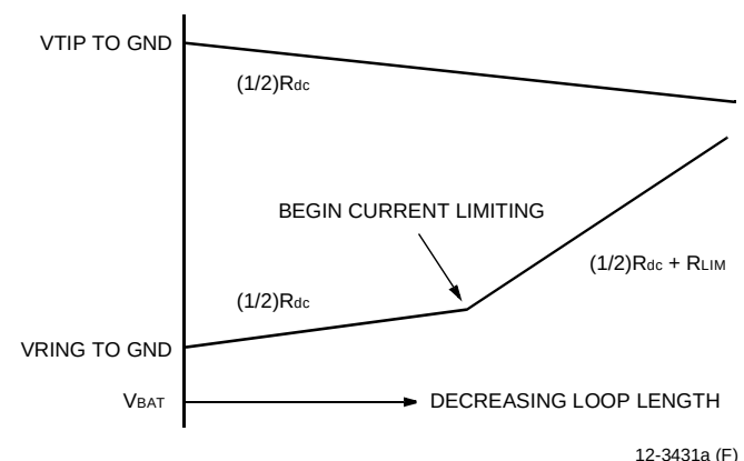
Figure 12. Tip/Ring Voltage
