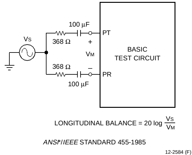
Figure 8. Longitudinal Balance
