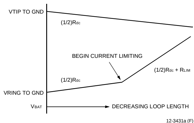
Figure 13. Tip/Ring Voltage
