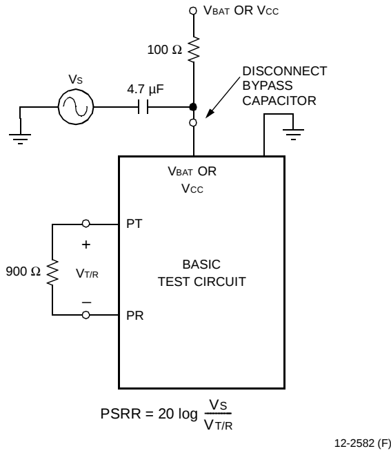
Figure 7. Metallic PSRR
