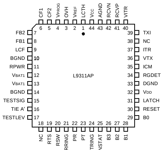
Figure 3. 44-Pin PLCC
