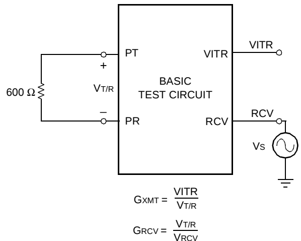
Figure 11. ac Gains
