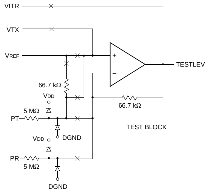
Figure 2. Test Diagram
