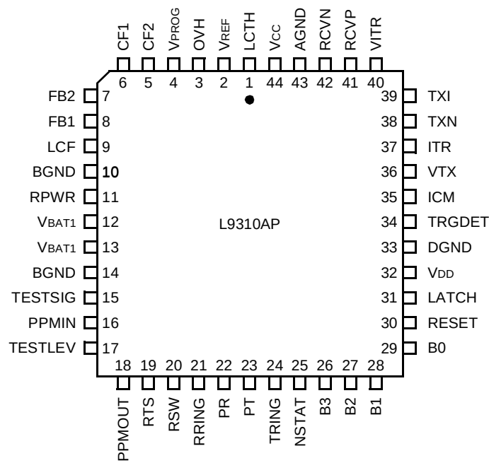
Figure 3. 44-Pin PLCC
