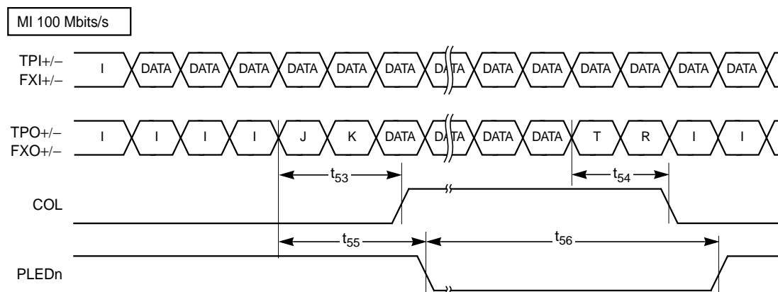
Figure 6.12 Collision Timing, Transmit (10 Mbits/s)
