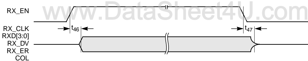
Figure 6.8 RX_EN Timing
