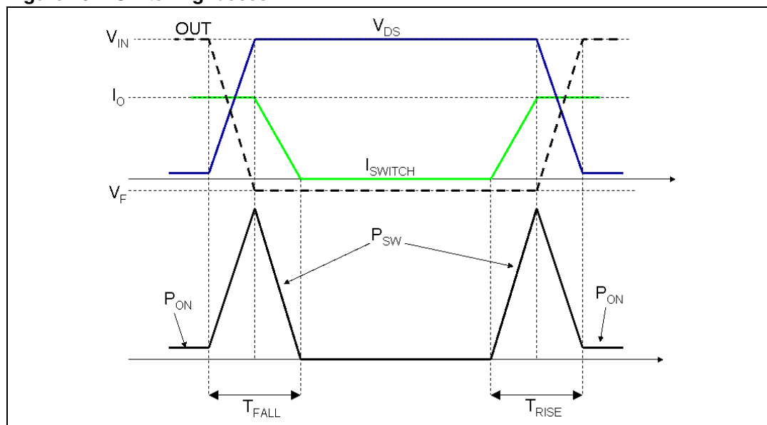
Figure 15. Switching losses
