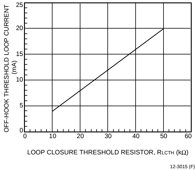
Figure 17. Loop Closure Program Resistor Selection
