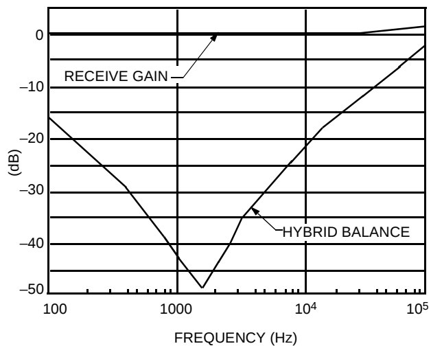
Figure 13. Receive Gain and Hybrid Balance vs. Frequency
