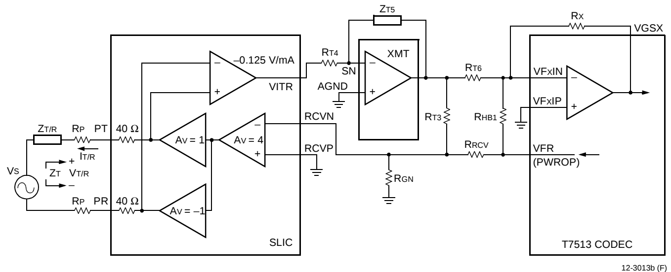
Figure 33. ac Equivalent Circuit Including Spare Op Amp
