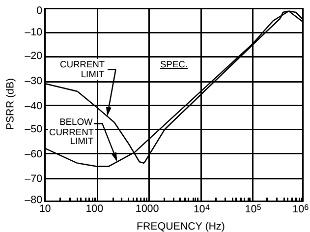
Figure 15. Typical V CC Power Supply Rejection
