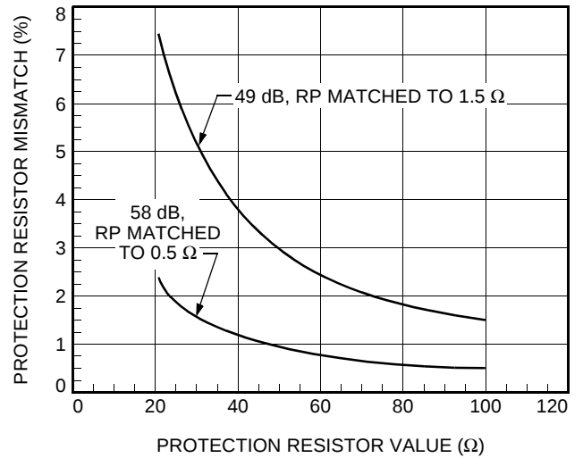
Figure 23. Longitudinal Balance Resistor Mismatch Requirements
