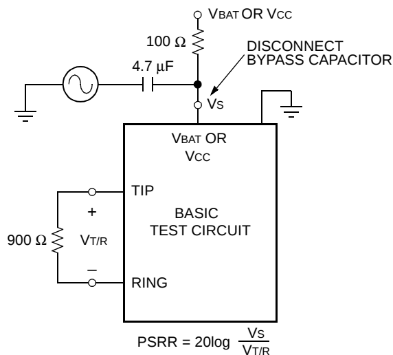
Figure 9. Metallic PSRR
