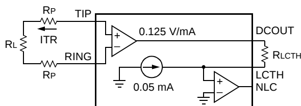
Figure 30. Off-Hook Detection Circuit Applications
