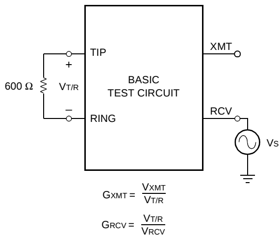
Figure 10. ac Gains
