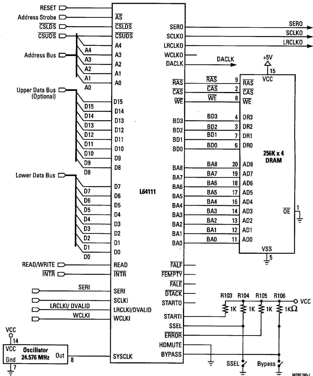
Figure 6.1 Application Using External Controller (Sheet 1 of 2)
