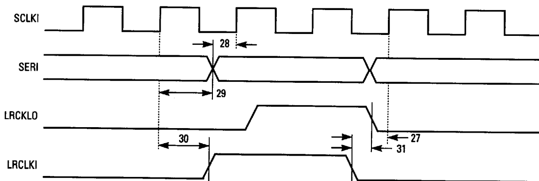
Figure 5.5 Input Timing
