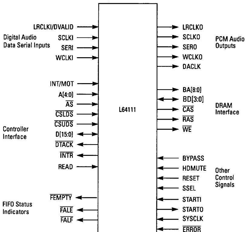
Figure 3.1 L64111 Logic Symbol
