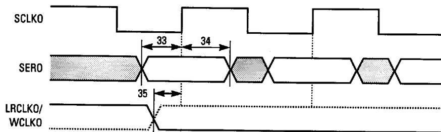
Figure 5.6 Serial PCM Data Out Timing
