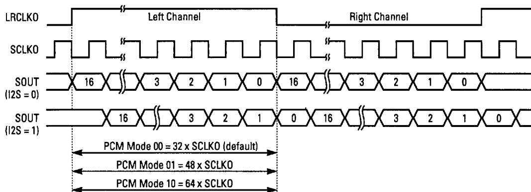
Figure 6.3 PCM Output Modes
