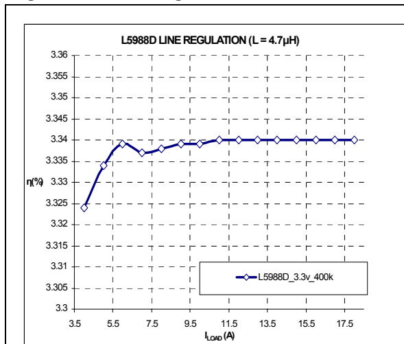
Figure 38. Line regulation
