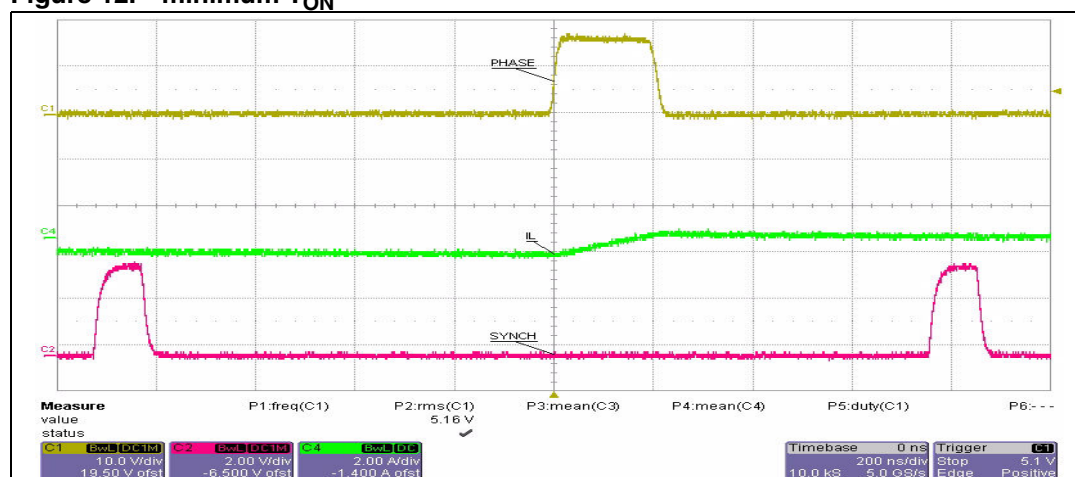
Figure 12. minimum T_{ON}
