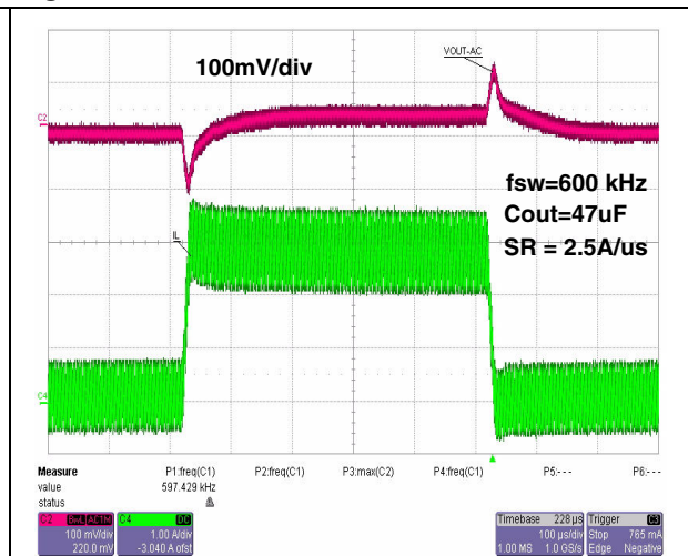
Figure 39. Load transient from 0 to 3 A
