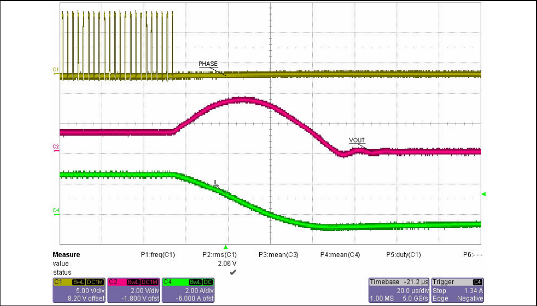
Figure 10. OVP latched
