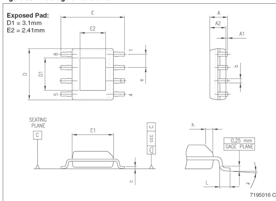
Figure 33. Package dimensions
