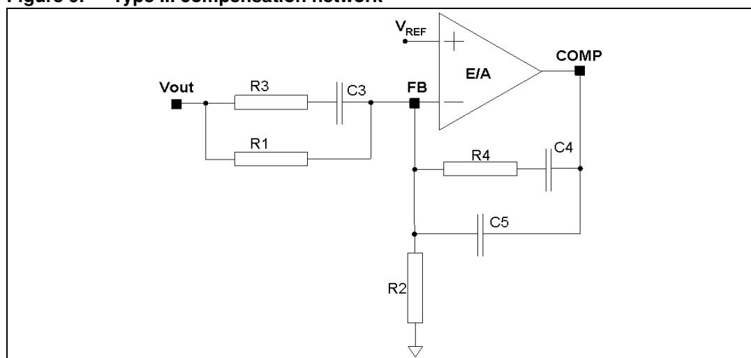
Figure 9. Type III compensation network
