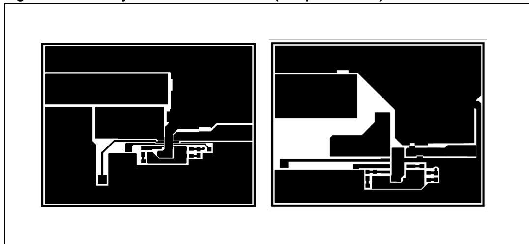
Figure 18. PCB layout: L5986 and L5986A (component side)
