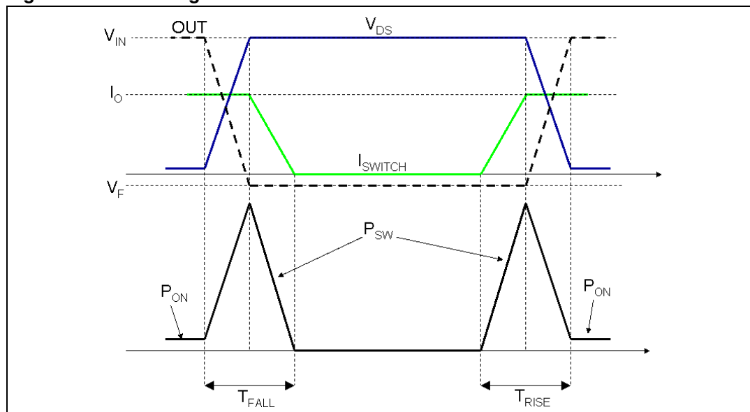
Figure 15. Switching losses
