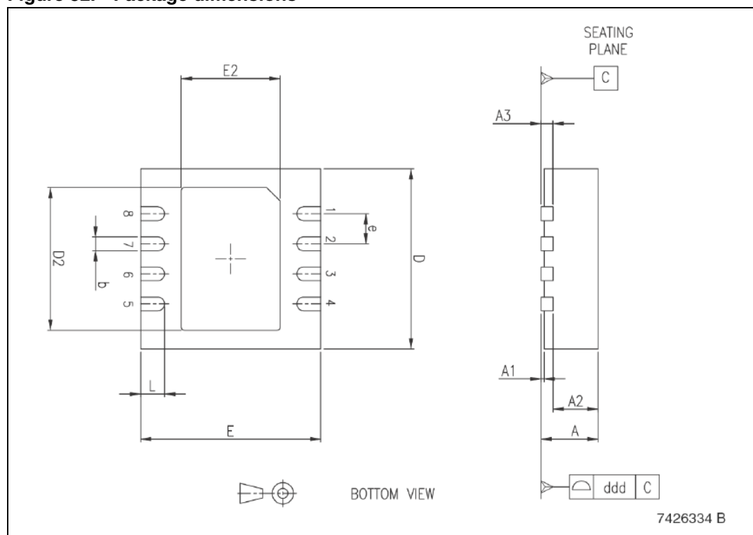
Figure 32. Package dimensions
