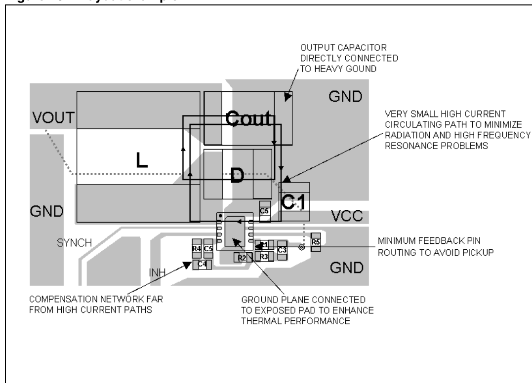
Figure 16. Layout example
