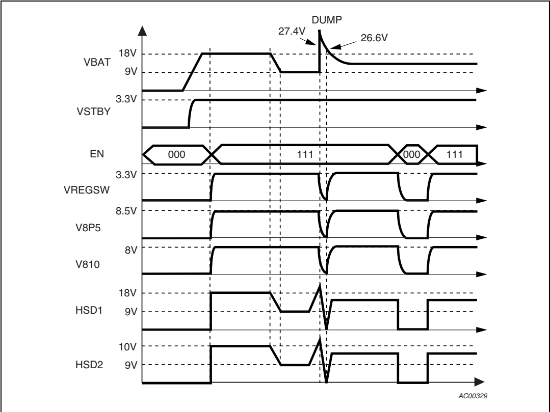
Figure 3. Timing diagram of regulators and HSD
