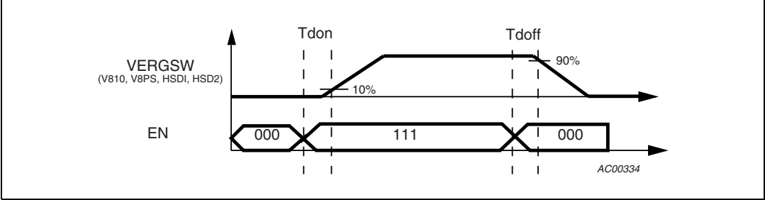
Figure 8. Enable on/off delay
