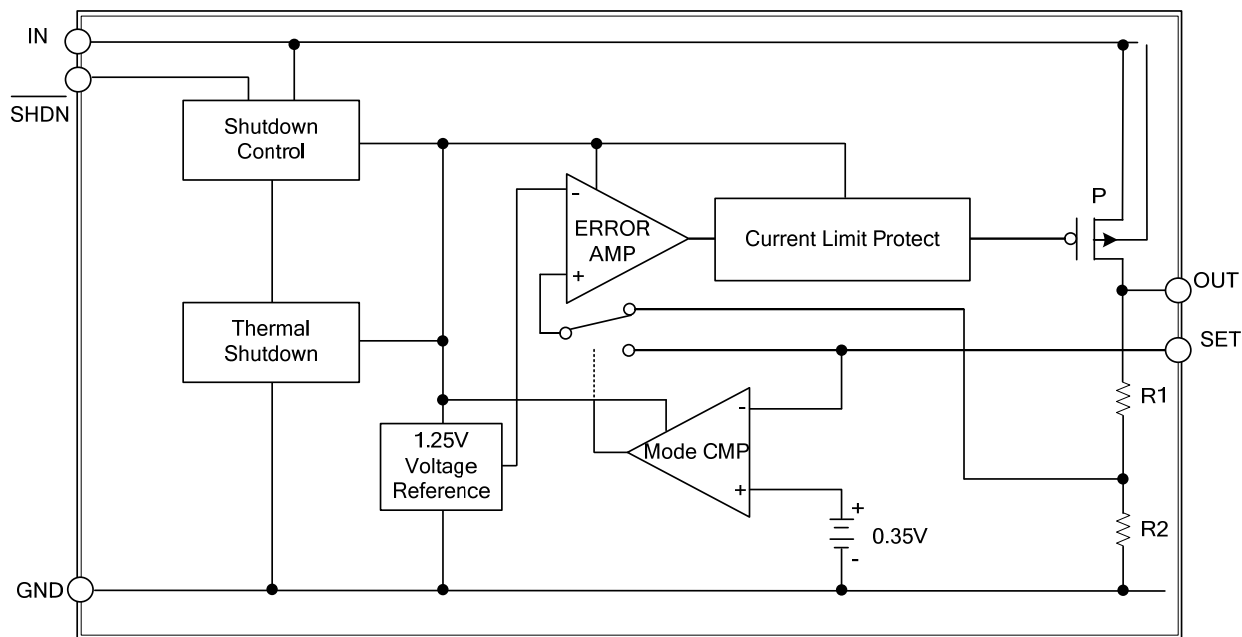
Figure 1. Functional Diagram
