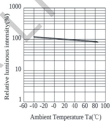
Fig.5 Luminous Intensity vs. Ambient Temperature
