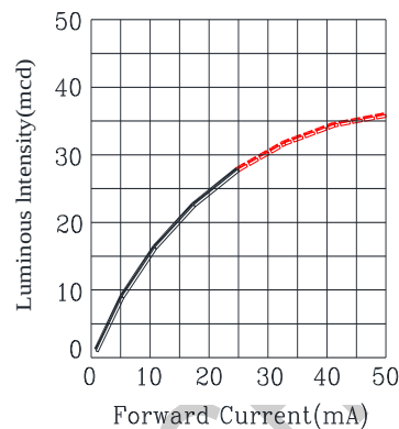
Fig.3 Luminous Intensity vs. Forward Current
