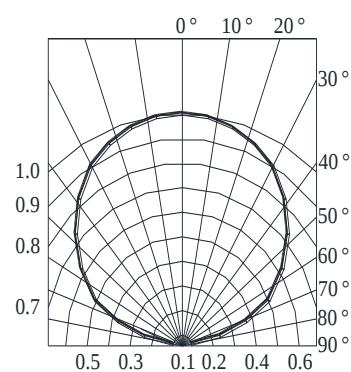
Fig.7 Relative Intensity vs. Angle
