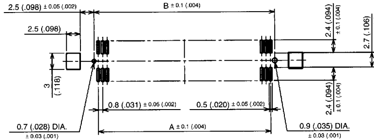
Applicable PCB Dimension (Ref.)
