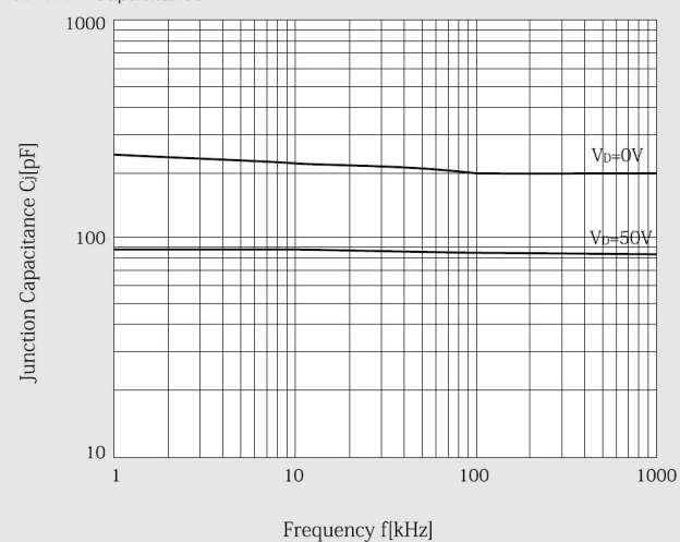
Junction Capacitance
