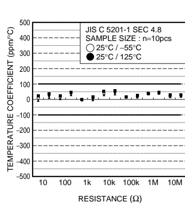
Fig.8 Variation resistance with temperature (F class)
