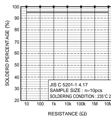
Fig.10 Solderability
