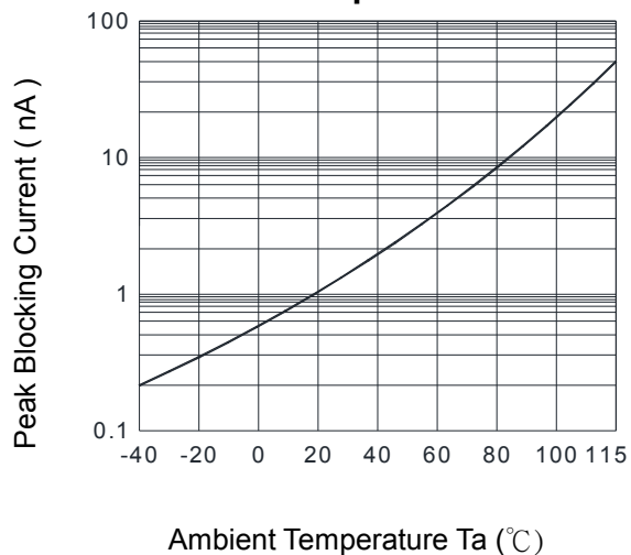
Fig.8 Leakage with LED off vs. Ambient Temperature
