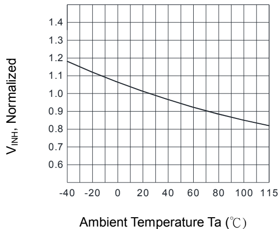
Fig.6 Inhibit Voltage vs. Ambient Temperature
