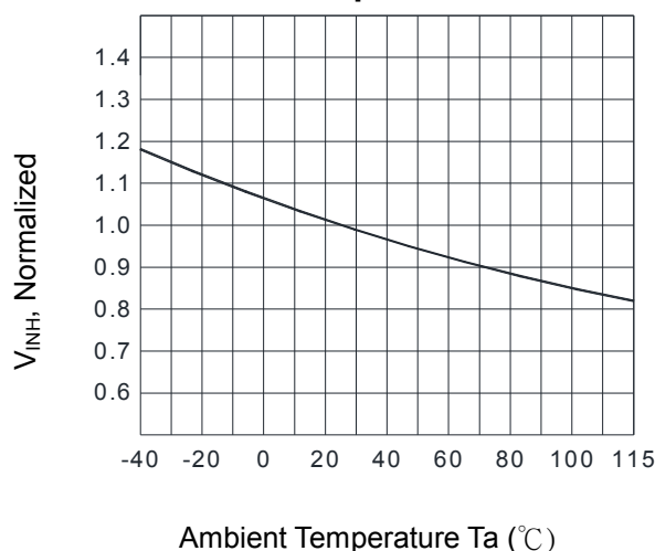
Fig.6 Inhibited Voltage V_{INH} vs. Ambient Temperature
