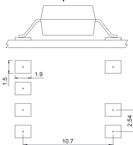
8-pin L
