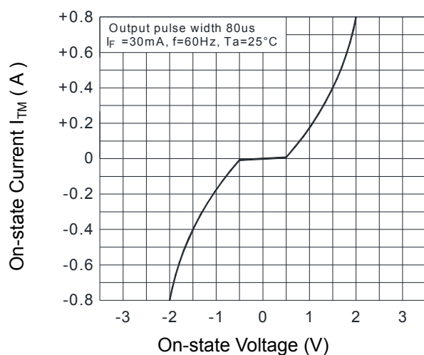
Fig.7 On-state Characteristics
