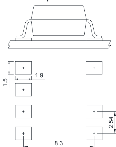
8-pin SMD
