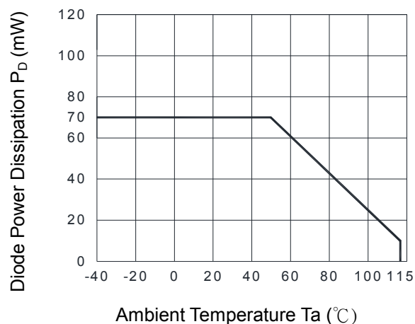
Fig.4 Total Power Dissipation P_D vs. Ambient Temperature
