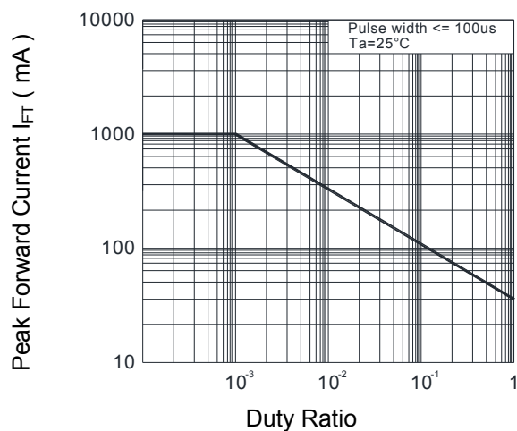
Fig.5 Peak Forward Current I_{FT} vs. Duty Ratio
