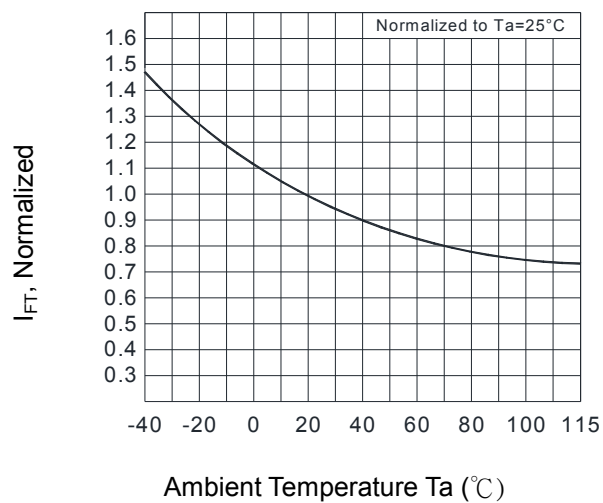
Fig.9 Trigger Current vs. Ambient Temperature
