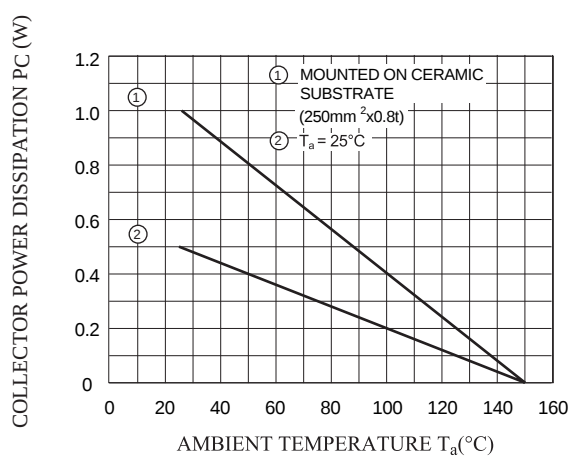
Fig.6 P_C - T_a
