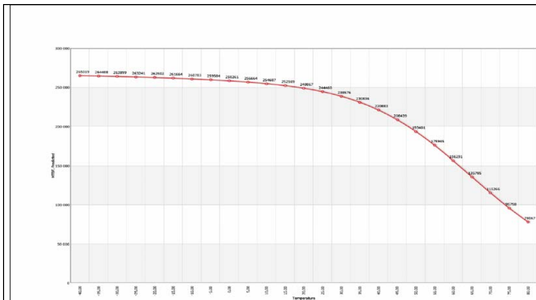
Figure 1. MTBF temperature de-rating.
