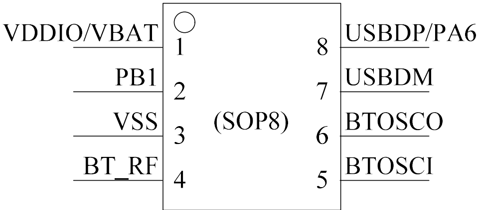
Figure 1-1 KT6368A Package Diagram
