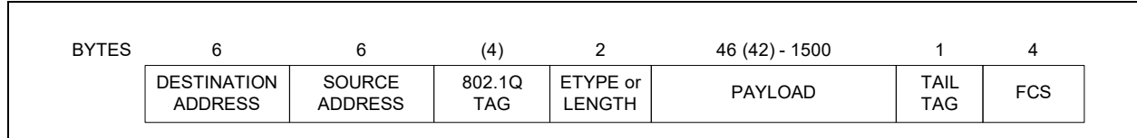
FIGURE 4-5: TAIL TAG FRAME FORMAT
