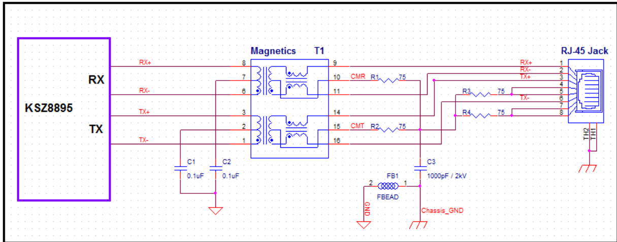
FIGURE 9-1: TWISTED PAIR INTERFACE
