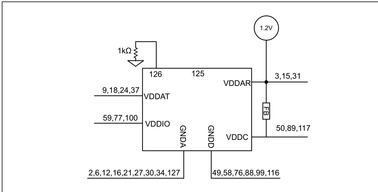
FIGURE 3-5: RECOMMENDED 1.2V POWER CONNECTION USING AN EXTERNAL 1.2V REGULATOR
