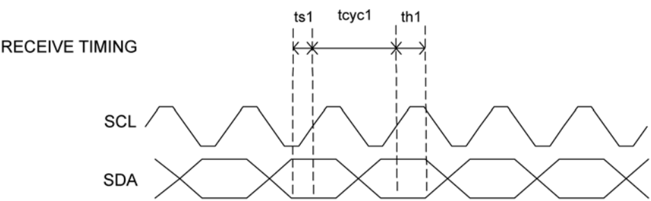
Figure 13. EEPROM Interface Input Receive Timing Diagram
