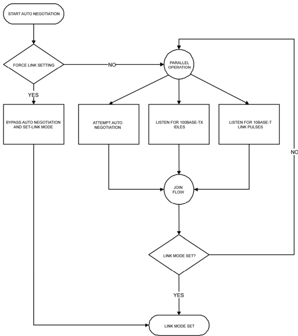
Figure 3. Auto-Negotiation
