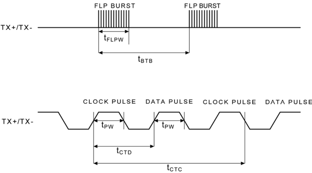
Figure 23. Auto-Negotiation Timing
