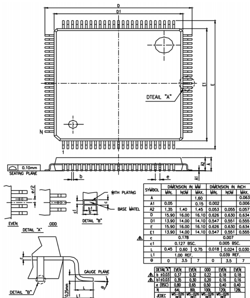
128-Pin LQFP
