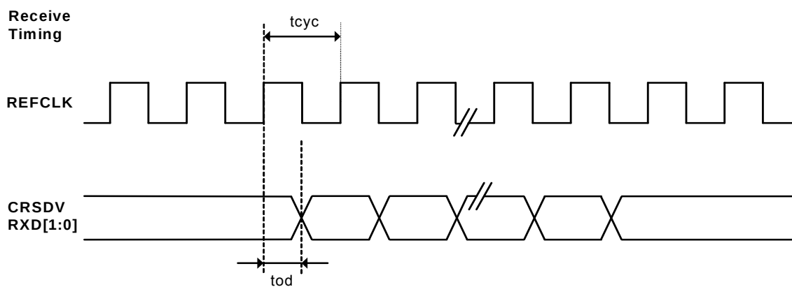
Figure 22. RMII Timing – Data Transmitted to RMII
