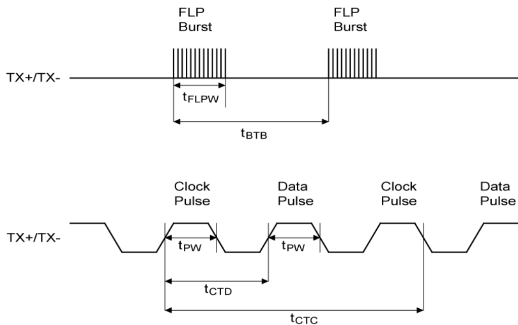
Figure 25: Auto-Negotiation Timing
