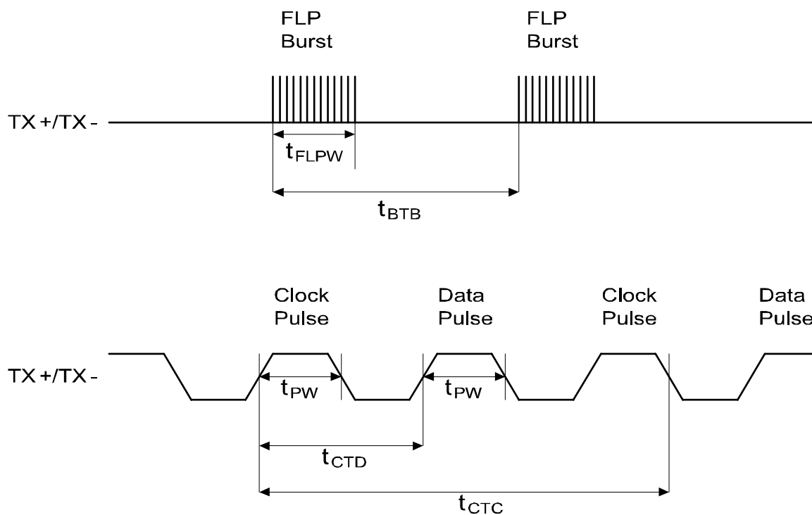
Figure 27. Auto-Negotiation Timing
