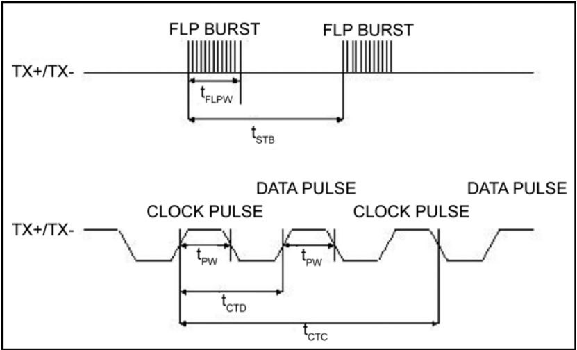
Figure 31. Auto-Negotiation Timing
