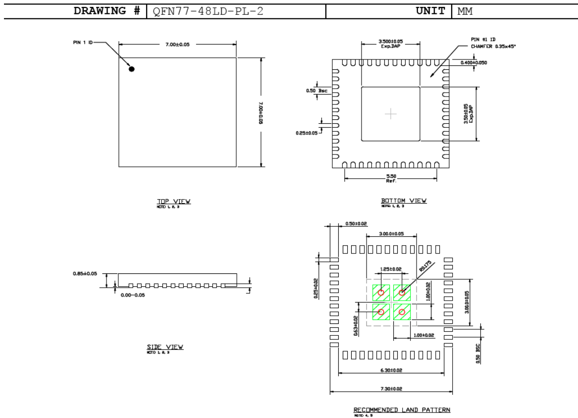
48 LEAD QFN 7x7mm PACKAGE OUTLINE & RECOMMENDED LAND PATTERN
