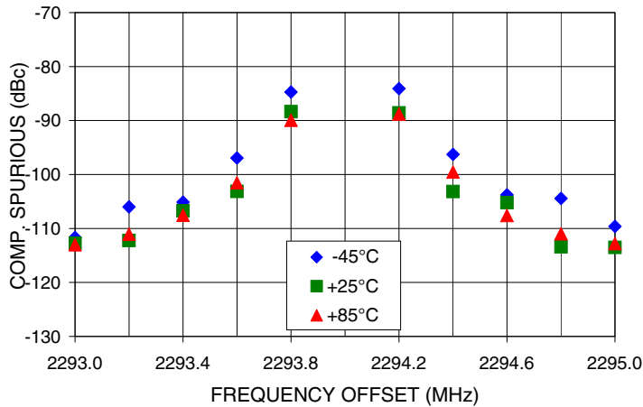
COMPARISON SPURIOUS Vs FREQ. OFFSET @ Fcar = 2294MHz
