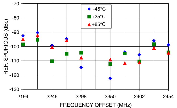
REFERENCE SPURIOUS Vs FREQ. OFFSET @ Fcar = 2324MHz
