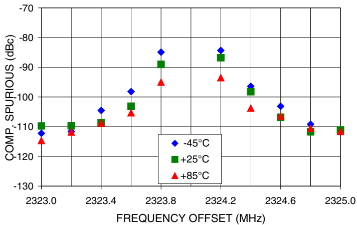
COMPARISON SPURIOUS Vs FREQ. OFFSET @ Fcar = 2324MHz
