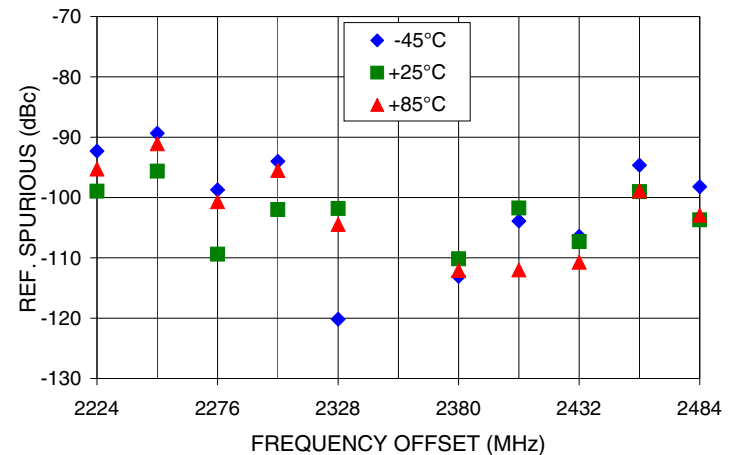
REFERENCE SPURIOUS Vs FREQ. OFFSET @ Fcar = 2354MHz
