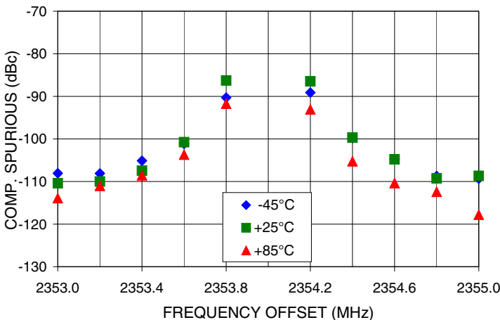
COMPARISON SPURIOUS Vs FREQ. OFFSET @ Fcar = 2354MHz
