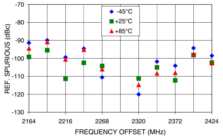
REFERENCE SPURIOUS Vs FREQ. OFFSET @ Fcar = 2294MHz
